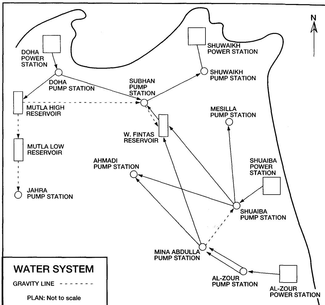
Figure 3—Water System
