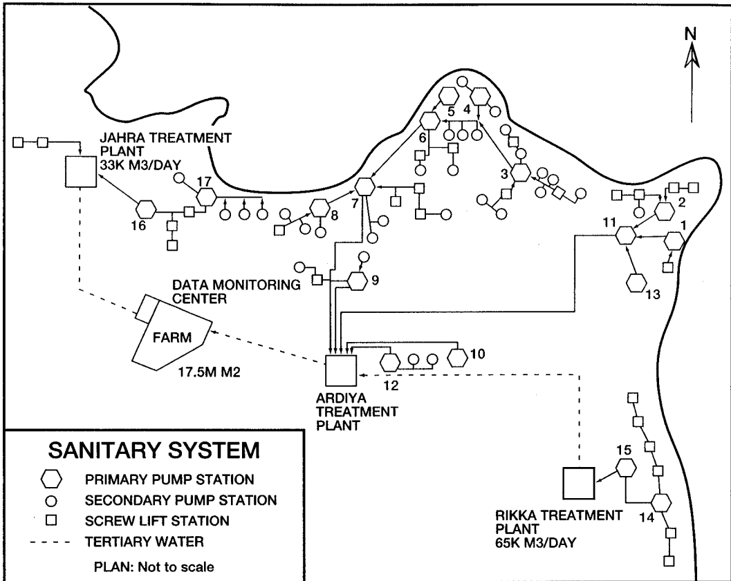
Figure 4—Sanitary System
